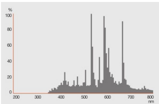
502825_HQI_TS_250W_WDL
