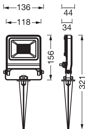
ENDURA GARDEN FLOOD 20W 830 SPIKE OSRAM
